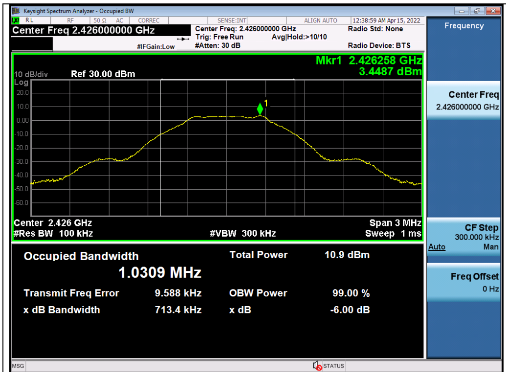
Test_Graph_LE1M_ANT1_2426_1Mbps_DTSBW
