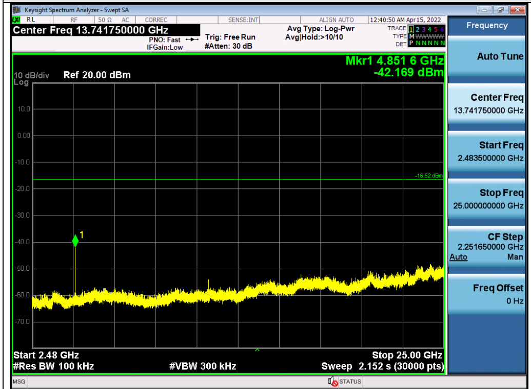
Test_Graph_LE1M_ANT1_2426_1Mbps_Higher Band Emissions
