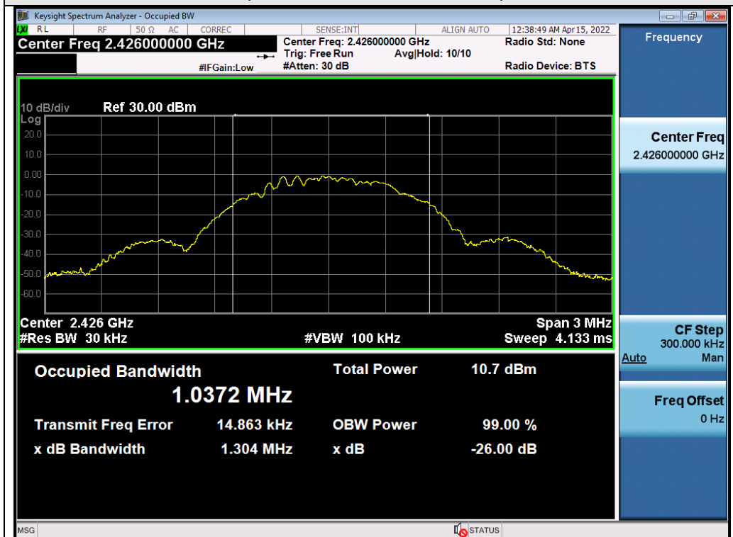
Test_Graph_LE1M_ANT1_2426_1Mbps_OBW
