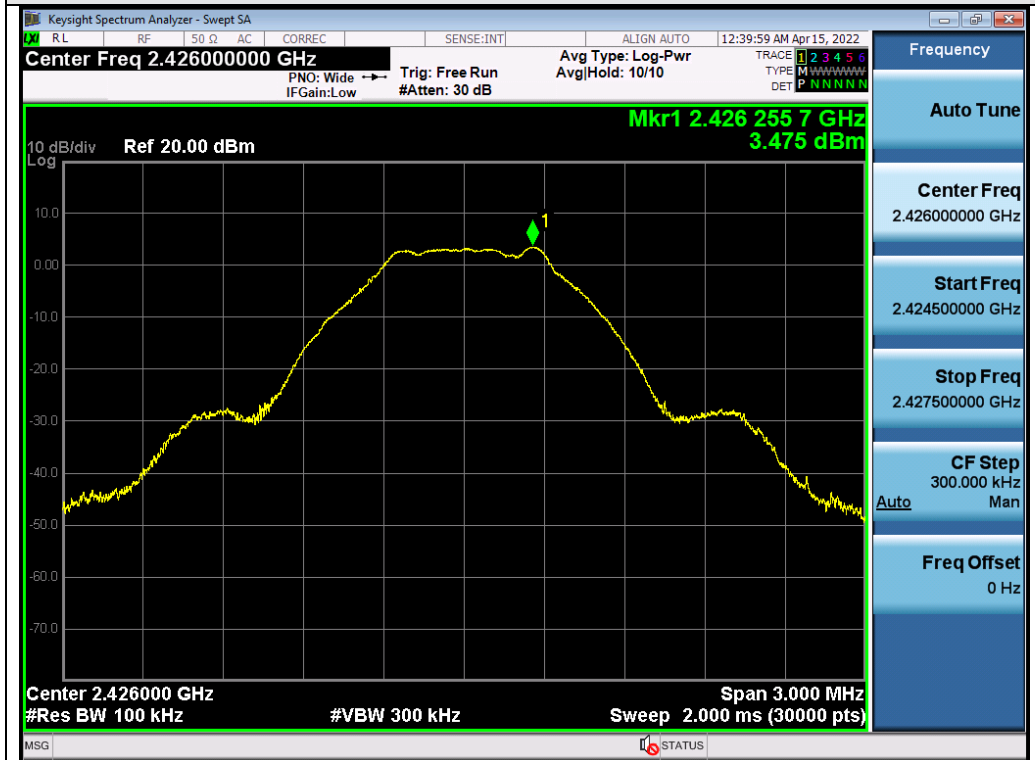
Test_Graph_LE1M_ANT1_2426_1Mbps_Reference Level
