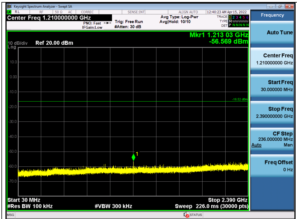
Test_Graph_LE1M_ANT1_2426_1Mbps_Lower Band Emissions
