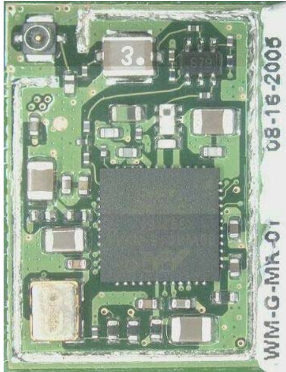
Top (without Shield)
