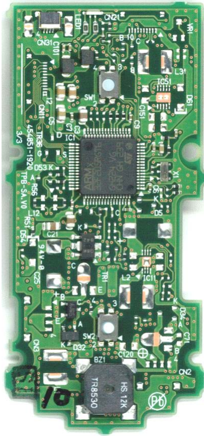
Fig. TOP View
