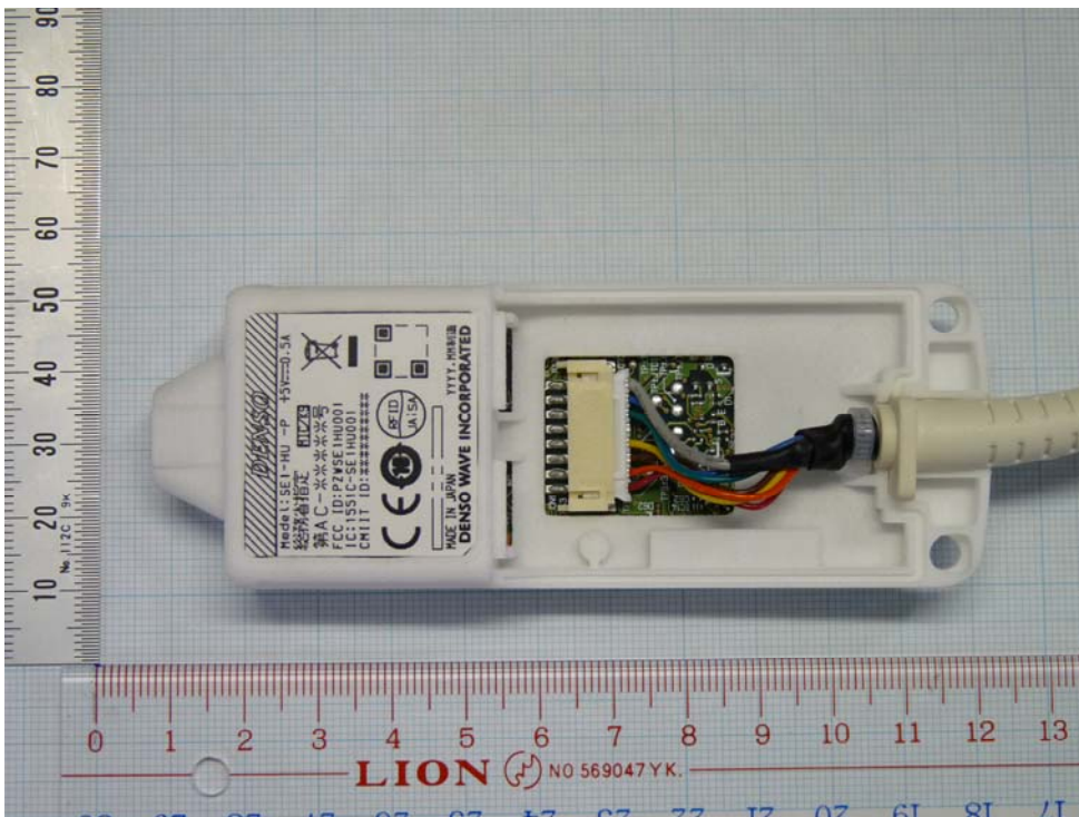
Fig. Internal Photo of SE1-HU (BOTTOM side)
