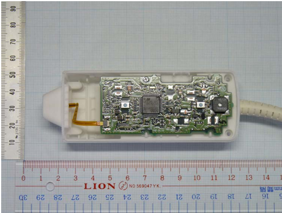
Fig. Internal Photo of SE1-HU (TOP side)
