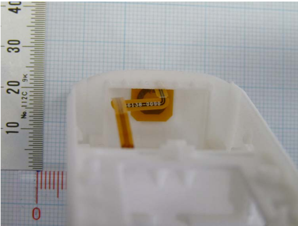
Fig. Internal Photo of SE1-HU (The antenna is stuck inside of the front part of case.)
