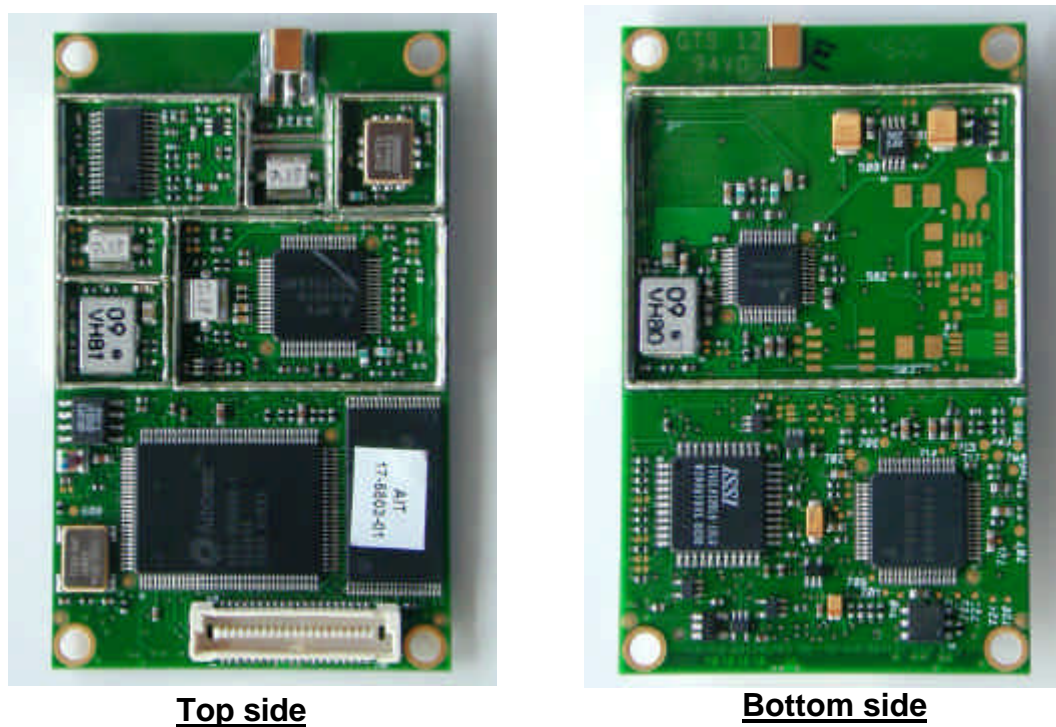
Fig 8.2. Appearance (without RF shield)
