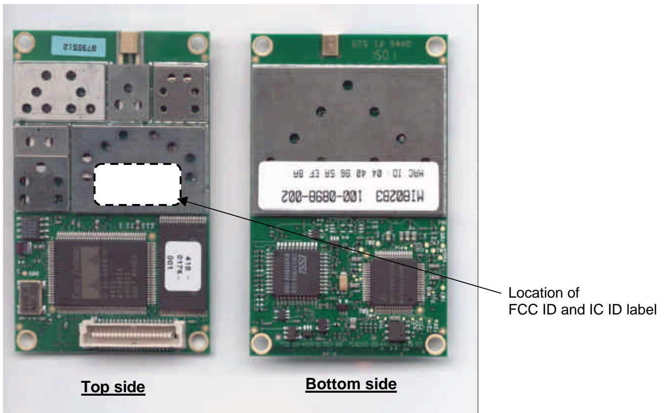
Fig 8.1. Appearance (with RF shield)
