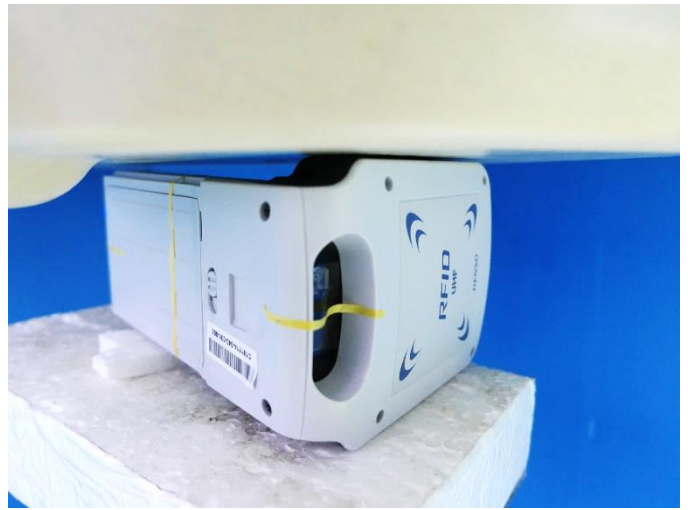
Fig-4.2 Right Side of EUT with 0 mm Gap
