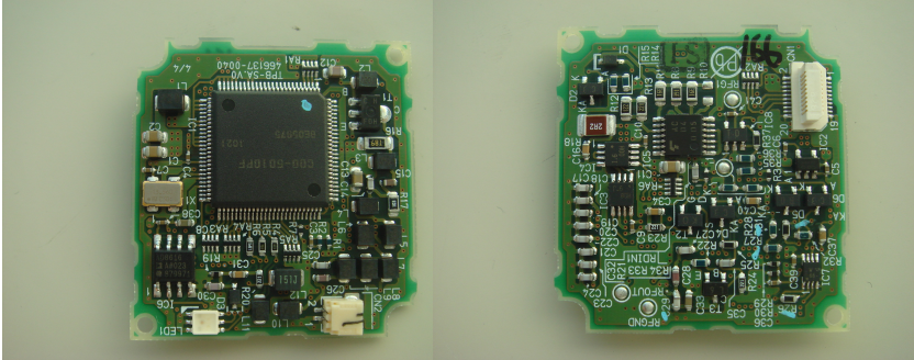
Main PCB (This PCB is the same as the Main PCB used in AN10R-01)
