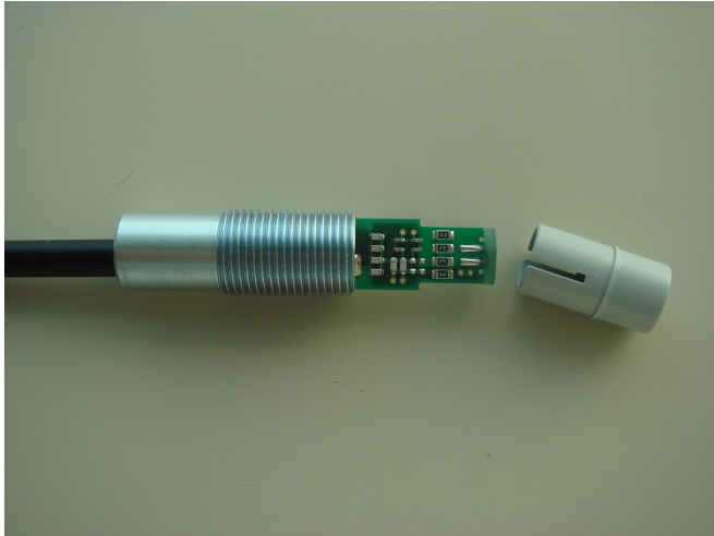
Antenna PCB sub assembly
