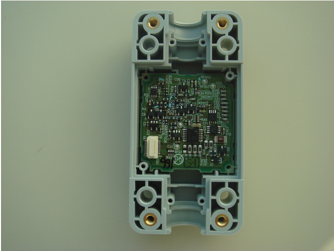
Main PCB sub assembly
