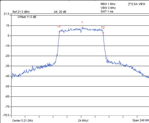
802.11ac (VHT80)_Chain 0 / CH42
