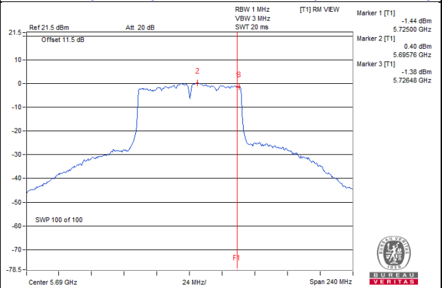
802.11ac (VHT80)_Chain 0 / CH138 (U-NII-2 Band)
