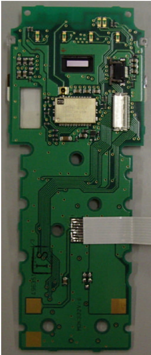
Component Side
