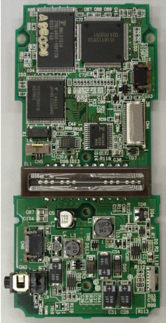
Solder Side
