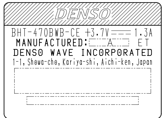
Rated Nameplate (BHT-470BWB-CE)
