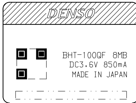
Rated Nameplate of BHT-100QF
