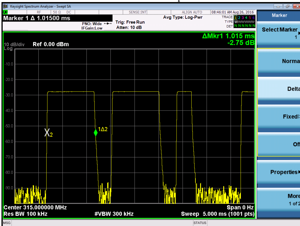
Dwell time of one pulse
