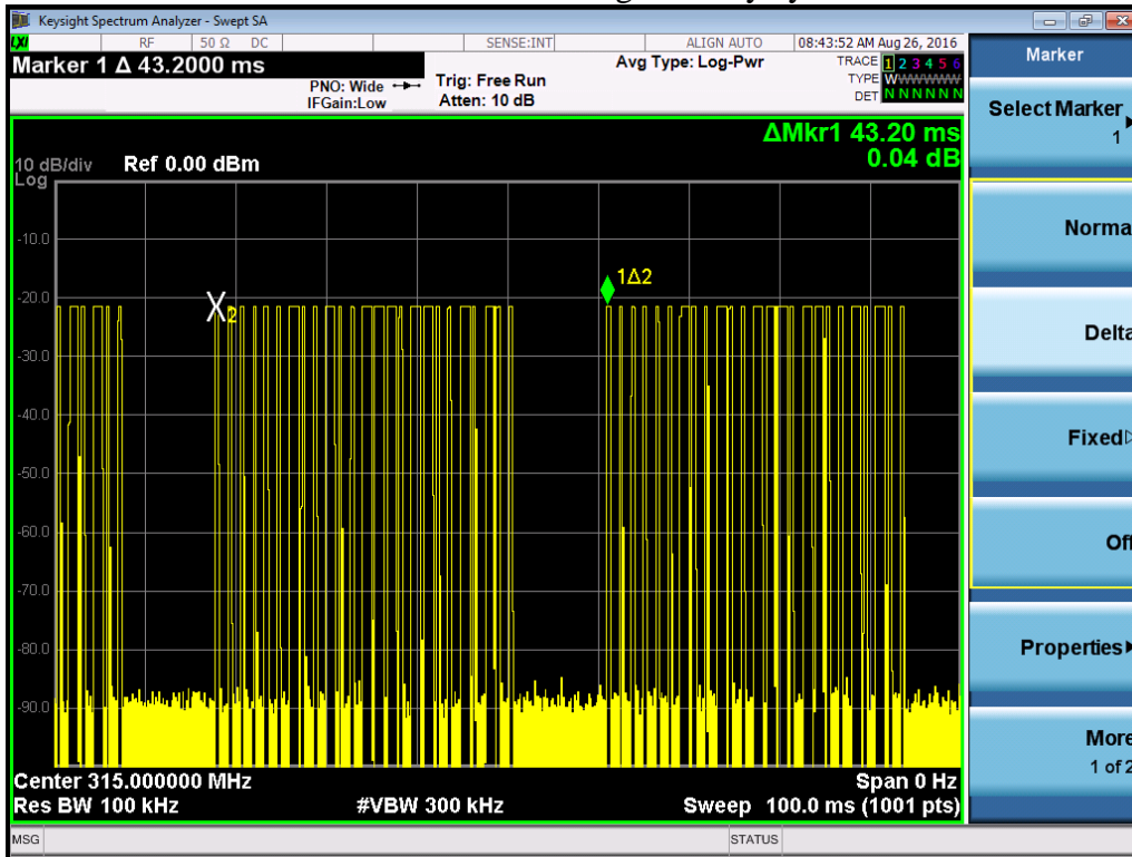
Pulse train with the highest duty cycle
