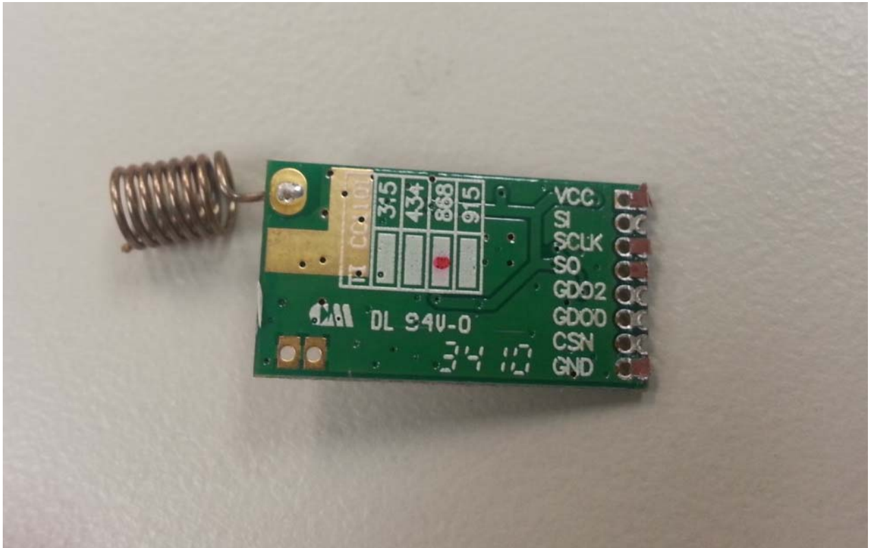
Photograph of RF Board: Foil Side
