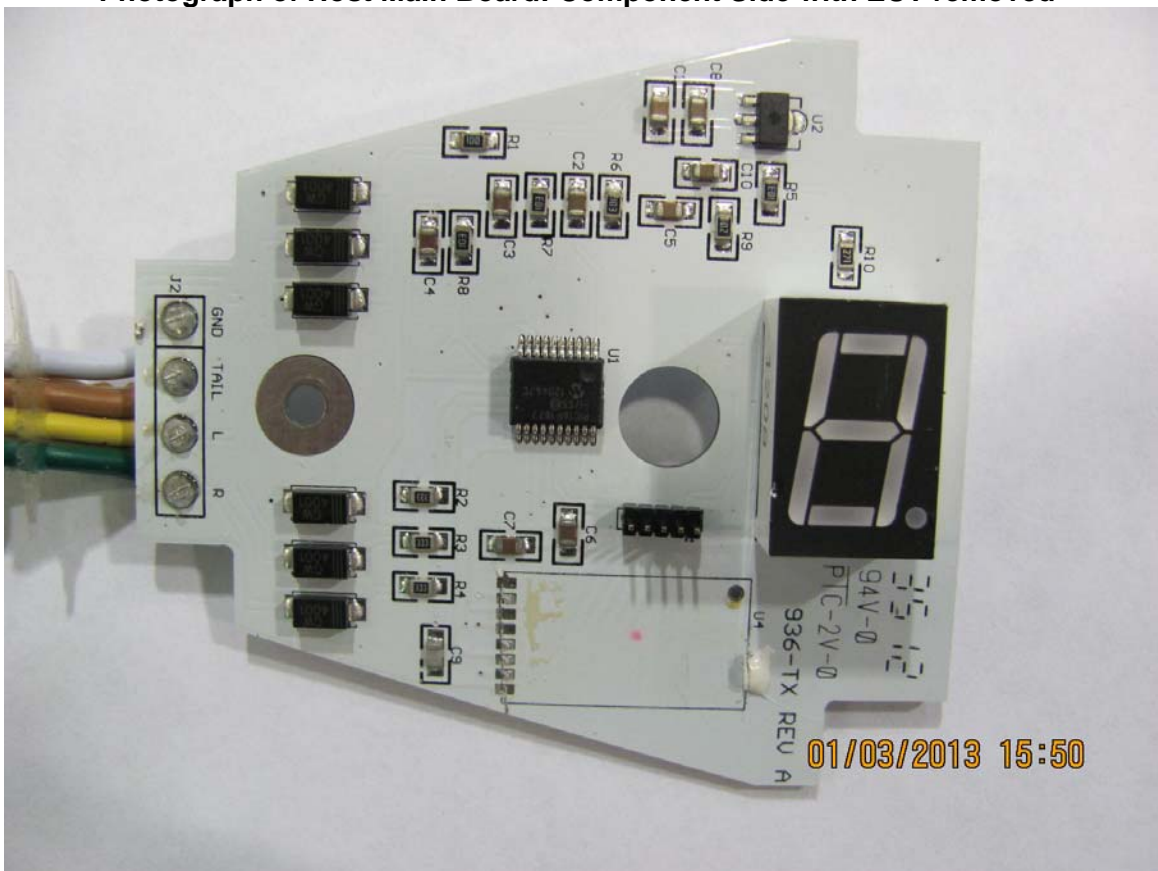
Photograph of Host Main Board: Component Side with EUT removed
