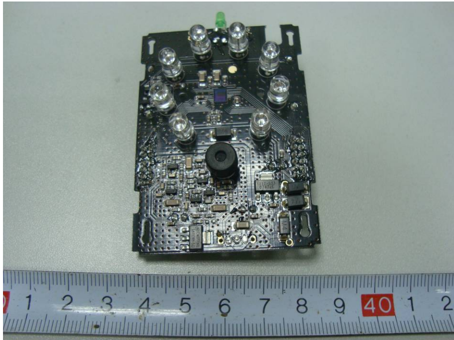
EUT – Camera Board Bottom Components View
