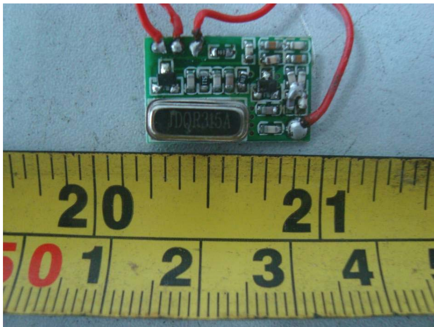
EUT- TX Board Components View
