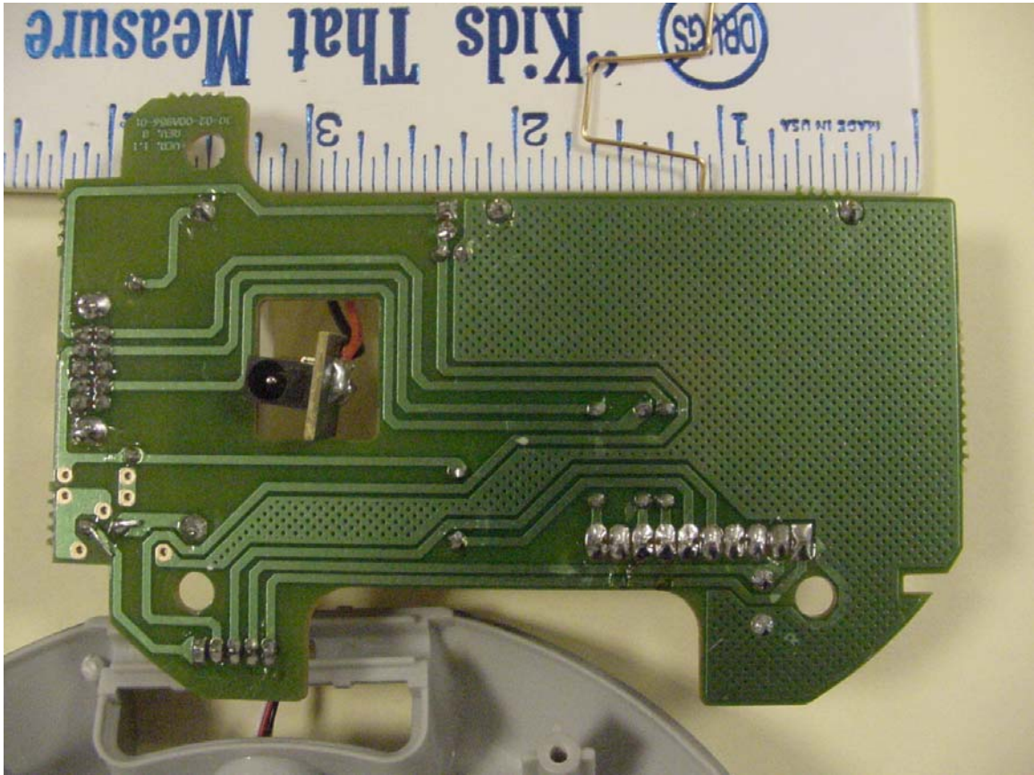
Rear/solder side of main PCB
