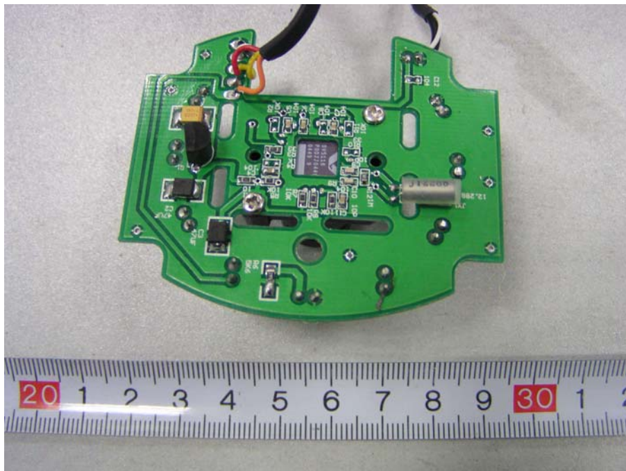
EUT-Camera PCB Rear View
