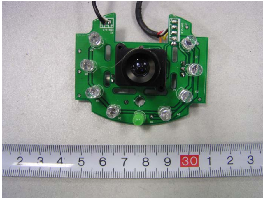
EUT-Camera PCB Front View
