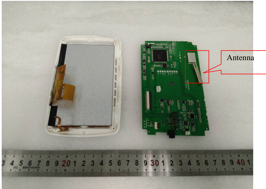
EUT – Cover off View 3
