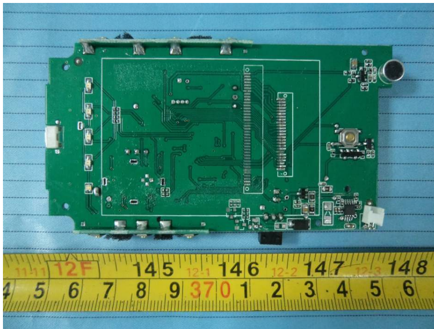
EUT – Main Board Bottom LCD Remove View
