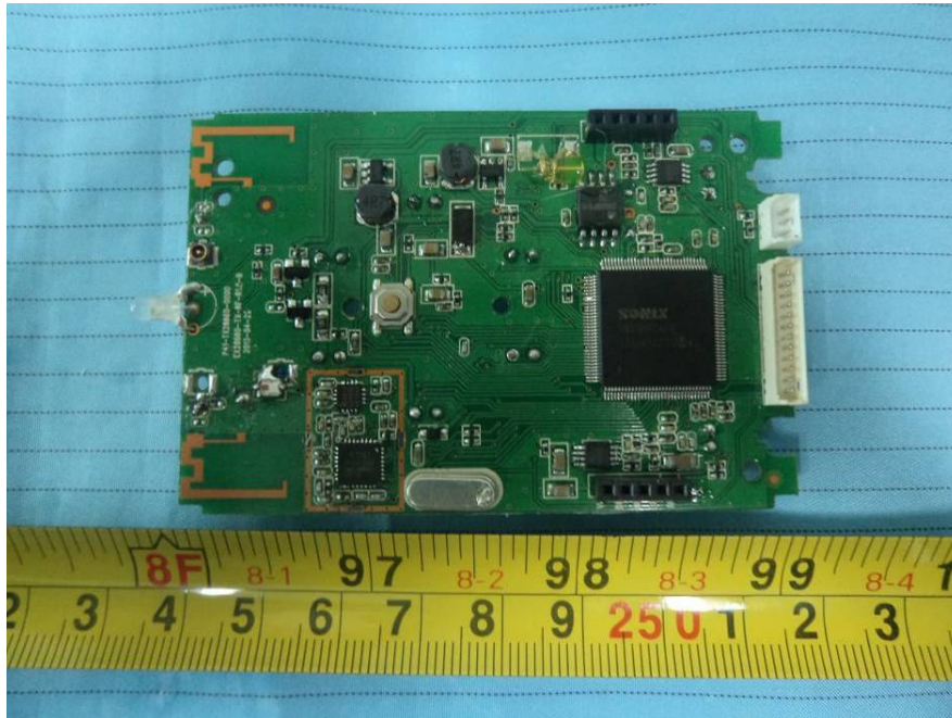
EUT – PCB Board 1 Top Shielding off View
