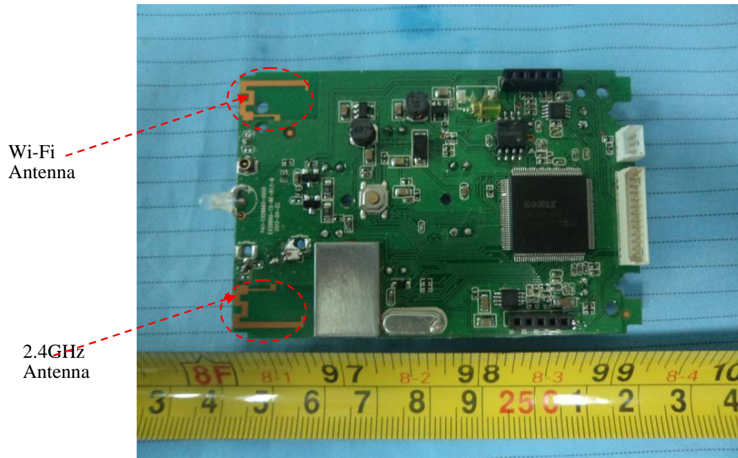
EUT – PCB Board 1 Top View
