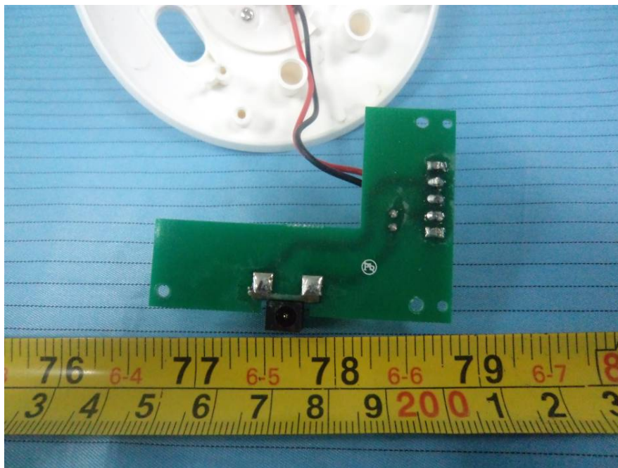
EUT – EX02040-PW-R1.0 Board Bottom View
