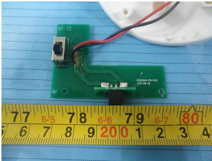
EUT – EX02040-PW-R1.0 Board Top View
