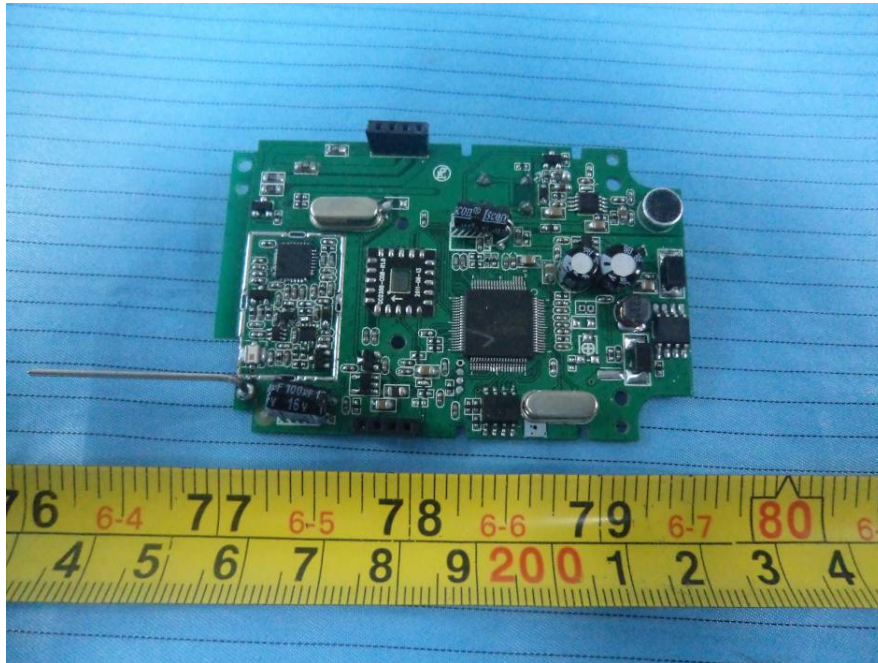
EUT – EX02040-RF-R1.0 Board Top View
