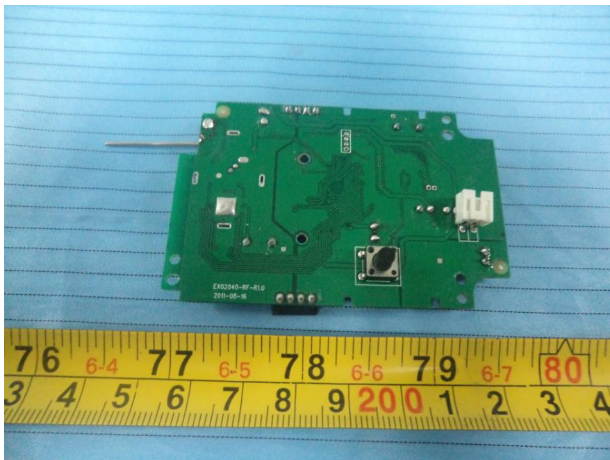
EUT – EX02040-RF-R1.0 Board Bottom View
