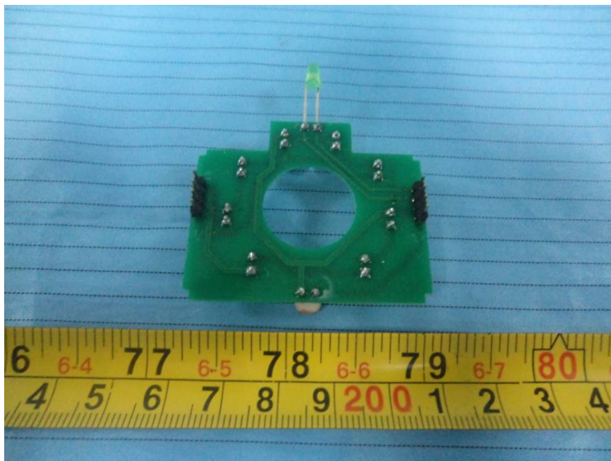
EUT – EX02040-LED-R1.0 Board Bottom View
