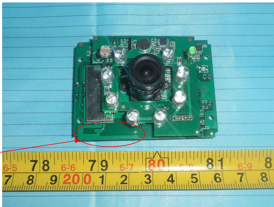
EUT – RF &LED Board View
