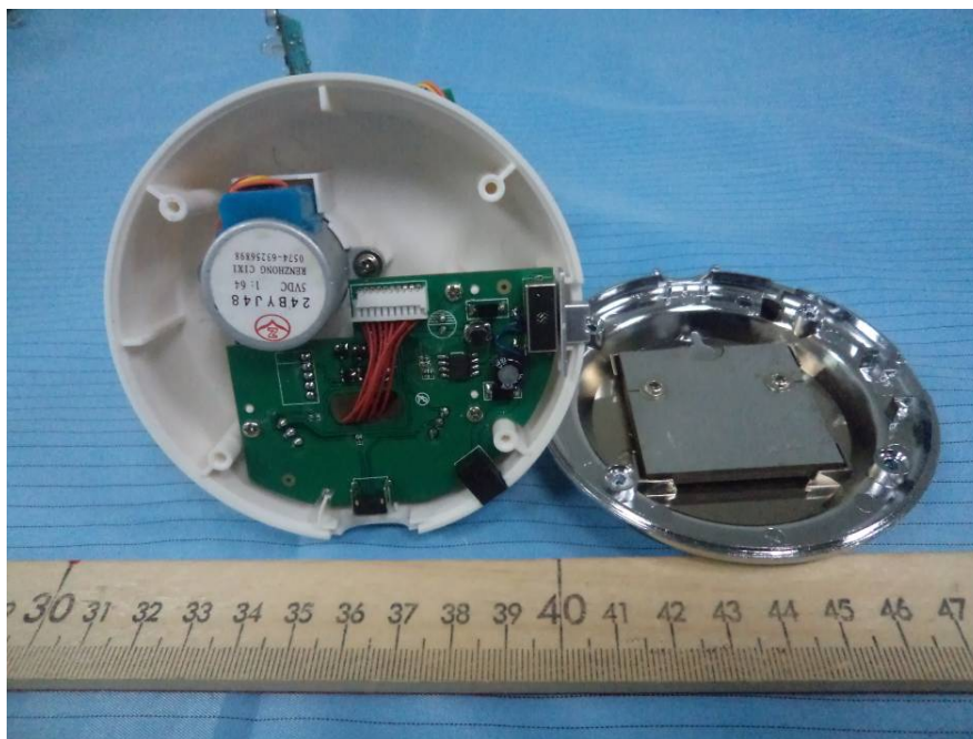
EUT – Power Board Cover off View
