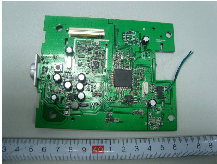
EUT – Main Board without Shielded Cover Top View
