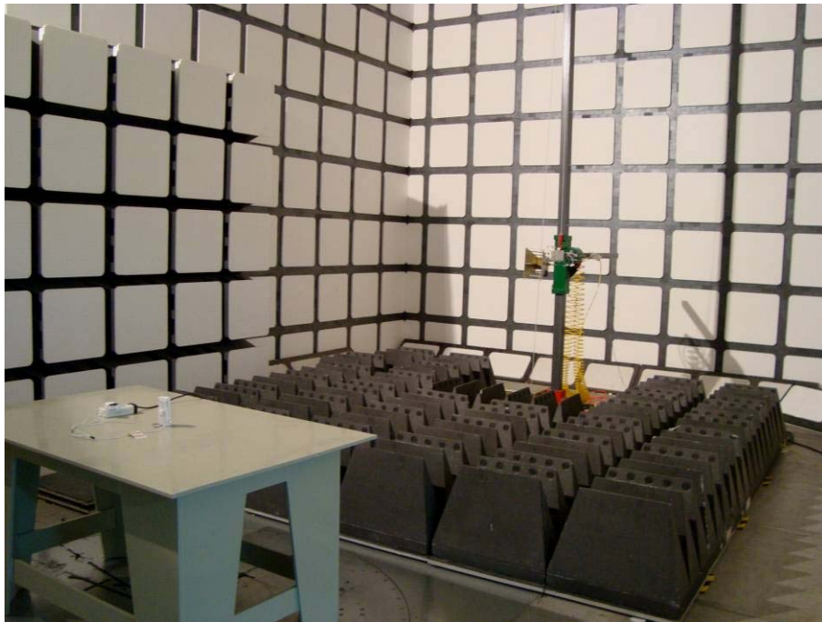
Above 1 GHz: Spurious Radiated Emissions with adapter- Rear View
