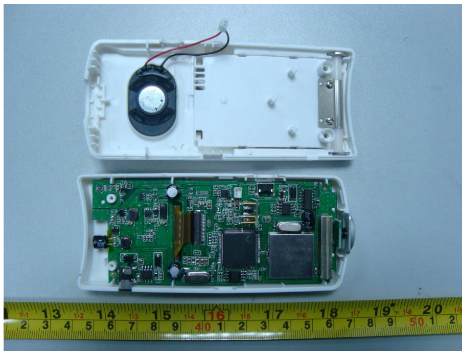
EUT – Main Board with LCD View
