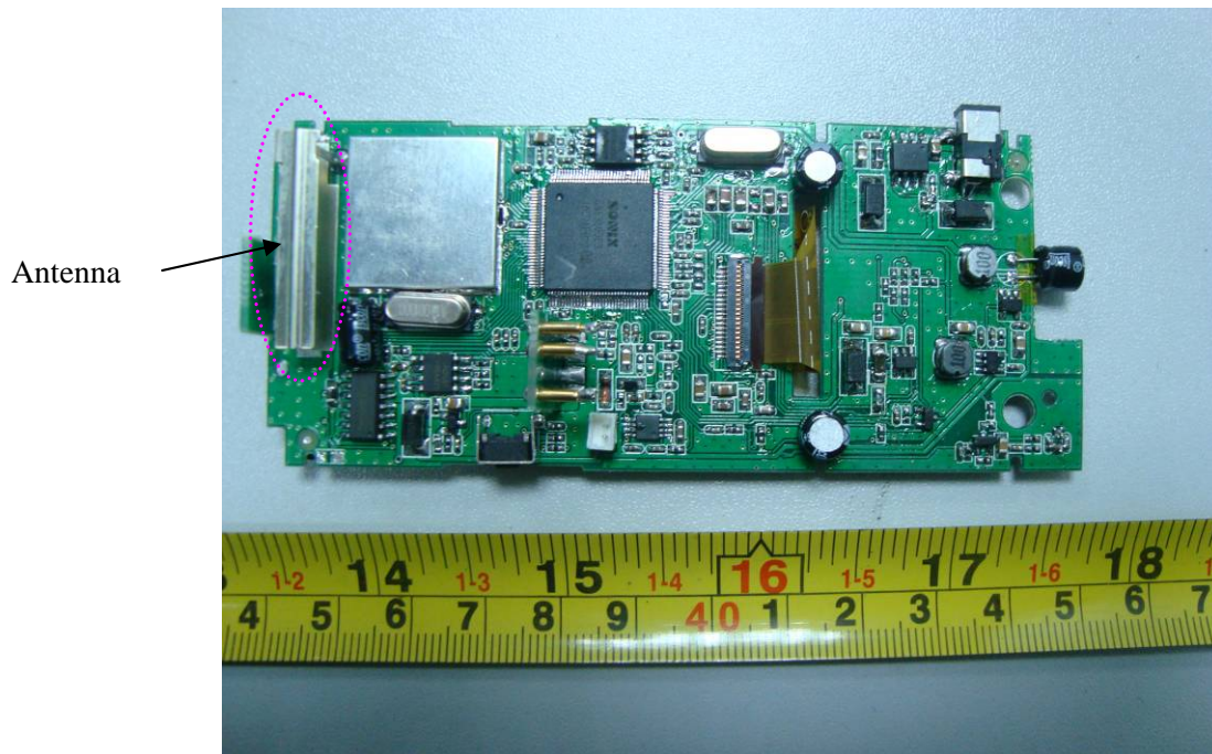
EUT – Power Board Shielding off Top View
