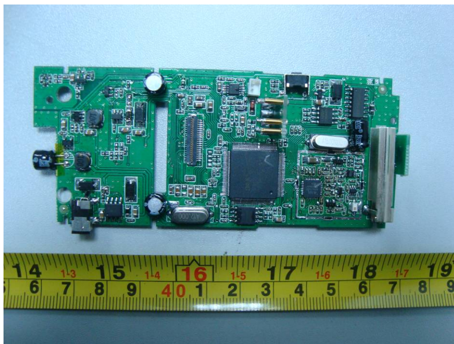
EUT – Power Board Shielding off Top View
