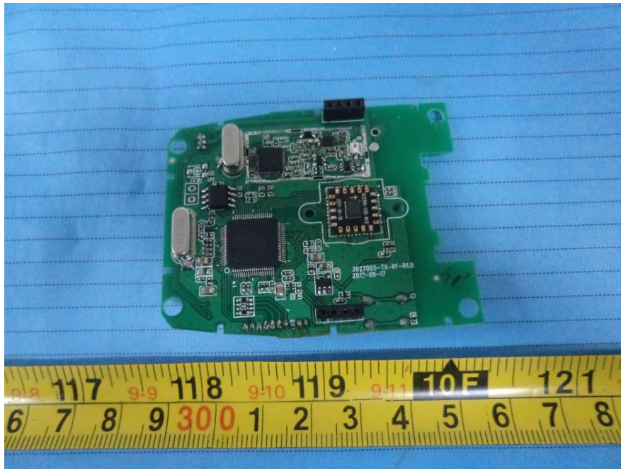
EUT – RF Board Shielding off View
