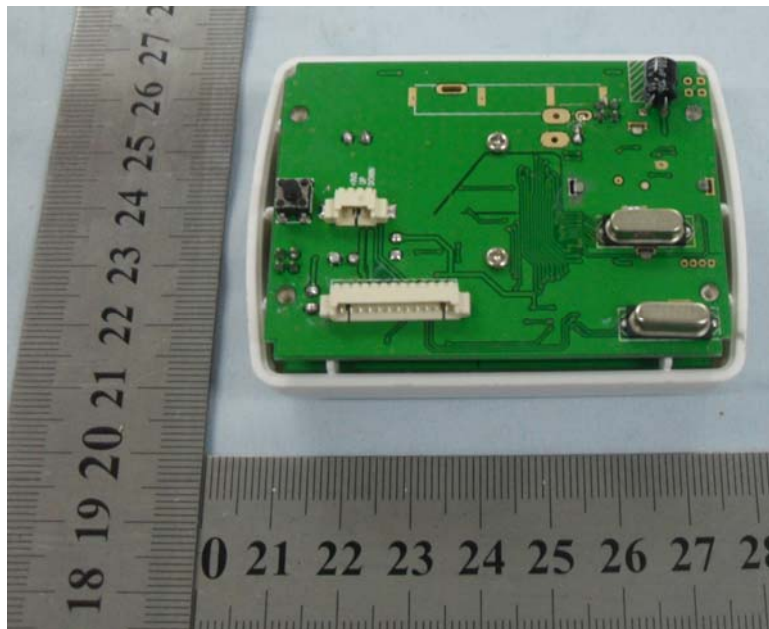
EUT - PCB View of Transmitter
