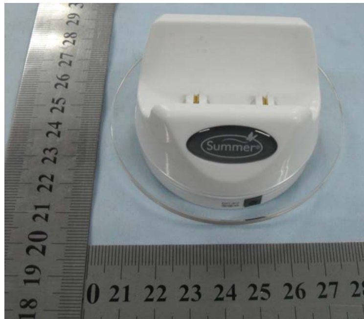
EUT – Receiver View base of receiver
