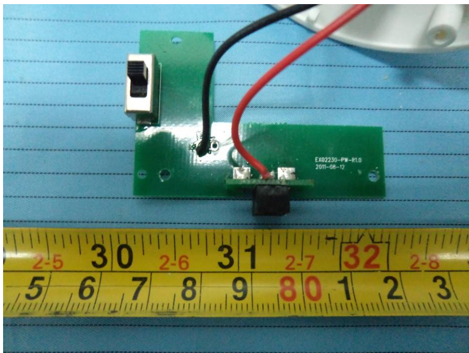
EUT – PW Board Top View
