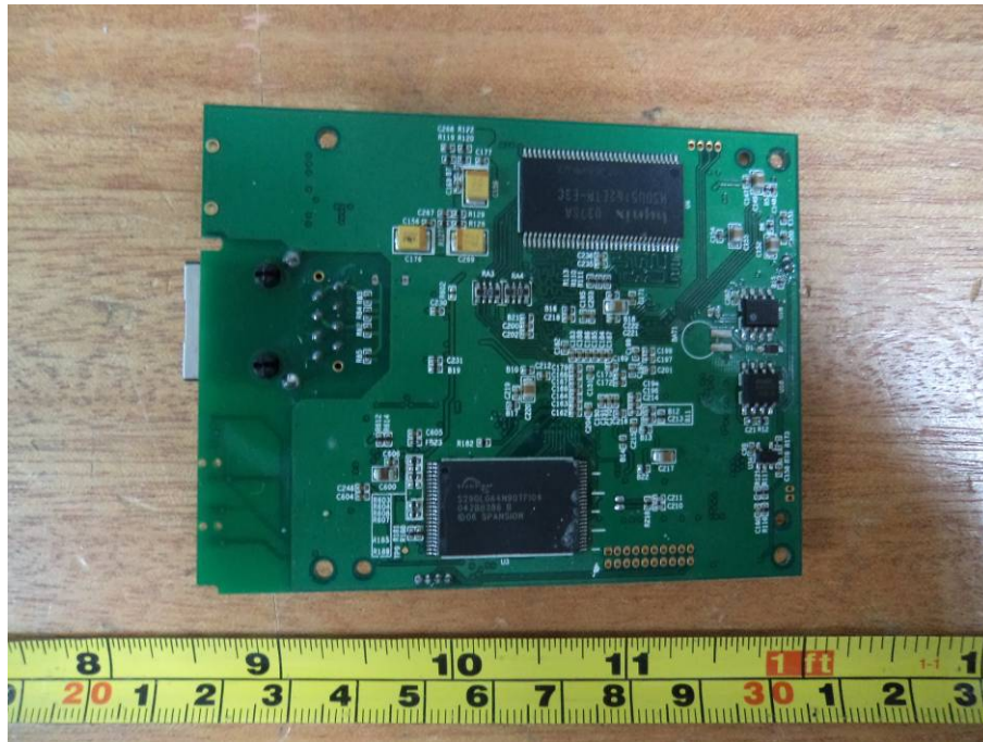
EUT – RF Board Top View 1
