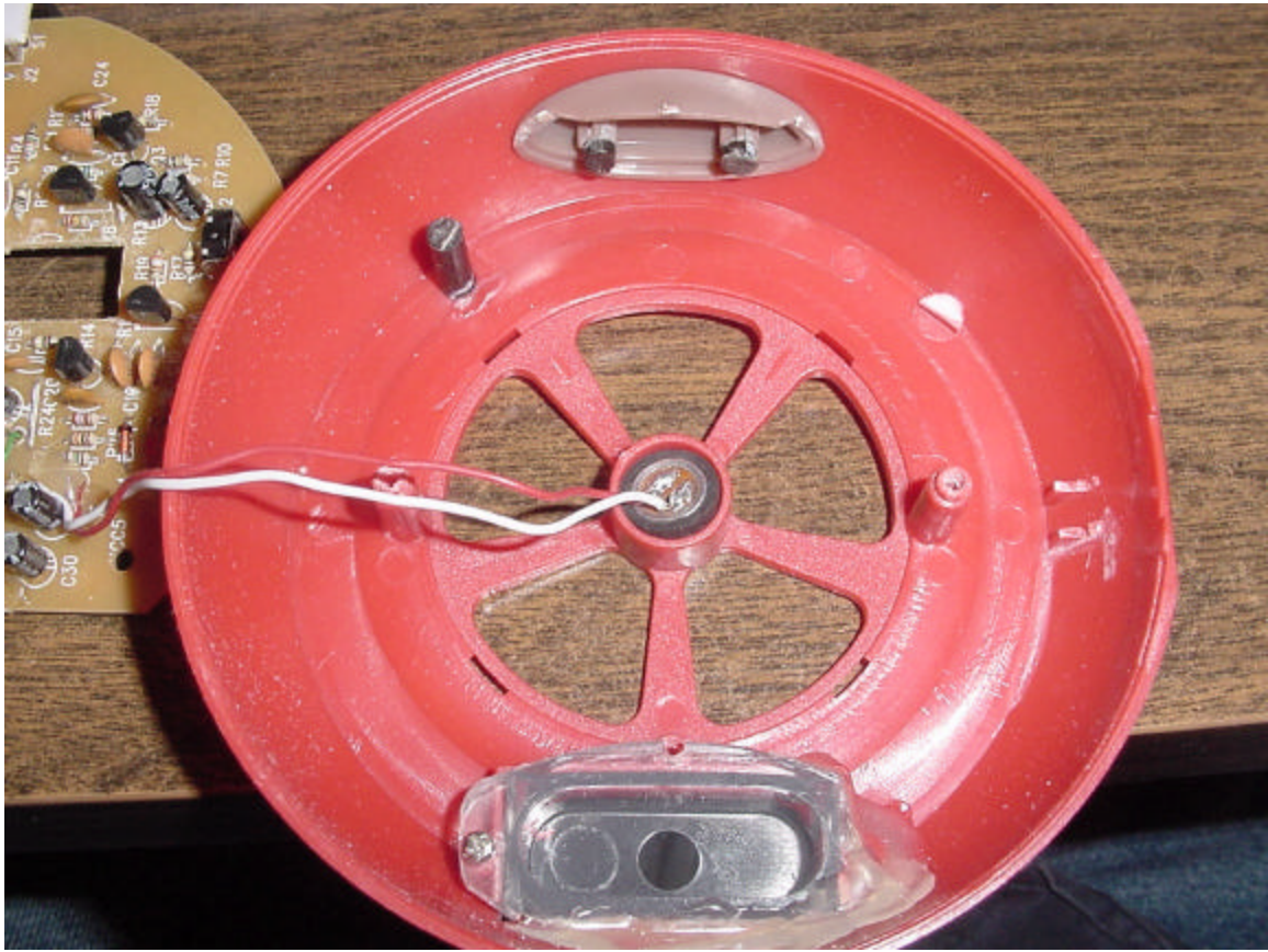
Inside of top housing with PCB removed, shows microphone.
