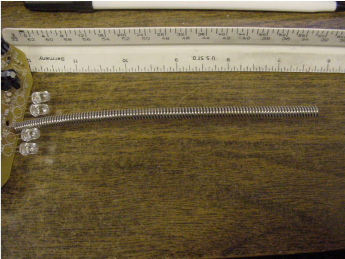
Photo showing antenna length (5.5")
