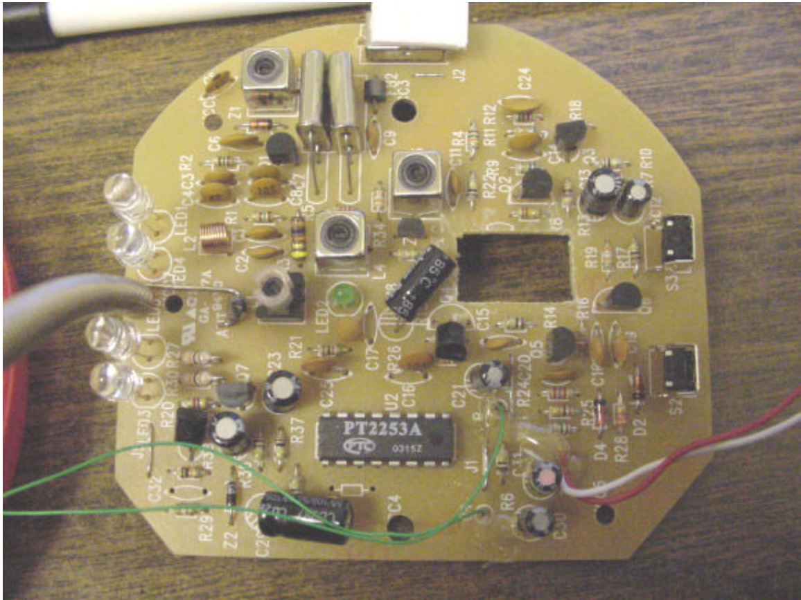
Component Side of PCB, shows permanently attached antenna (soldered)
