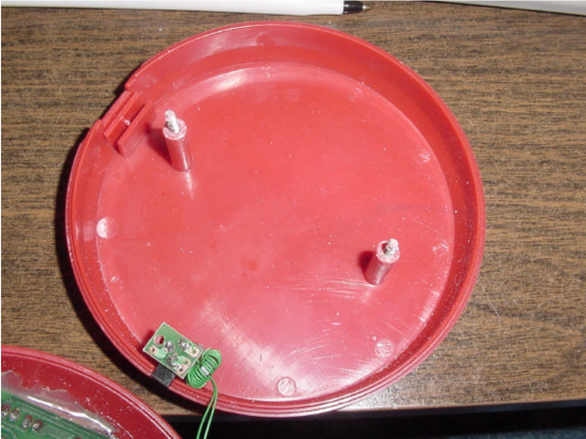
Inside of base, showing the power jack and a small choke.
