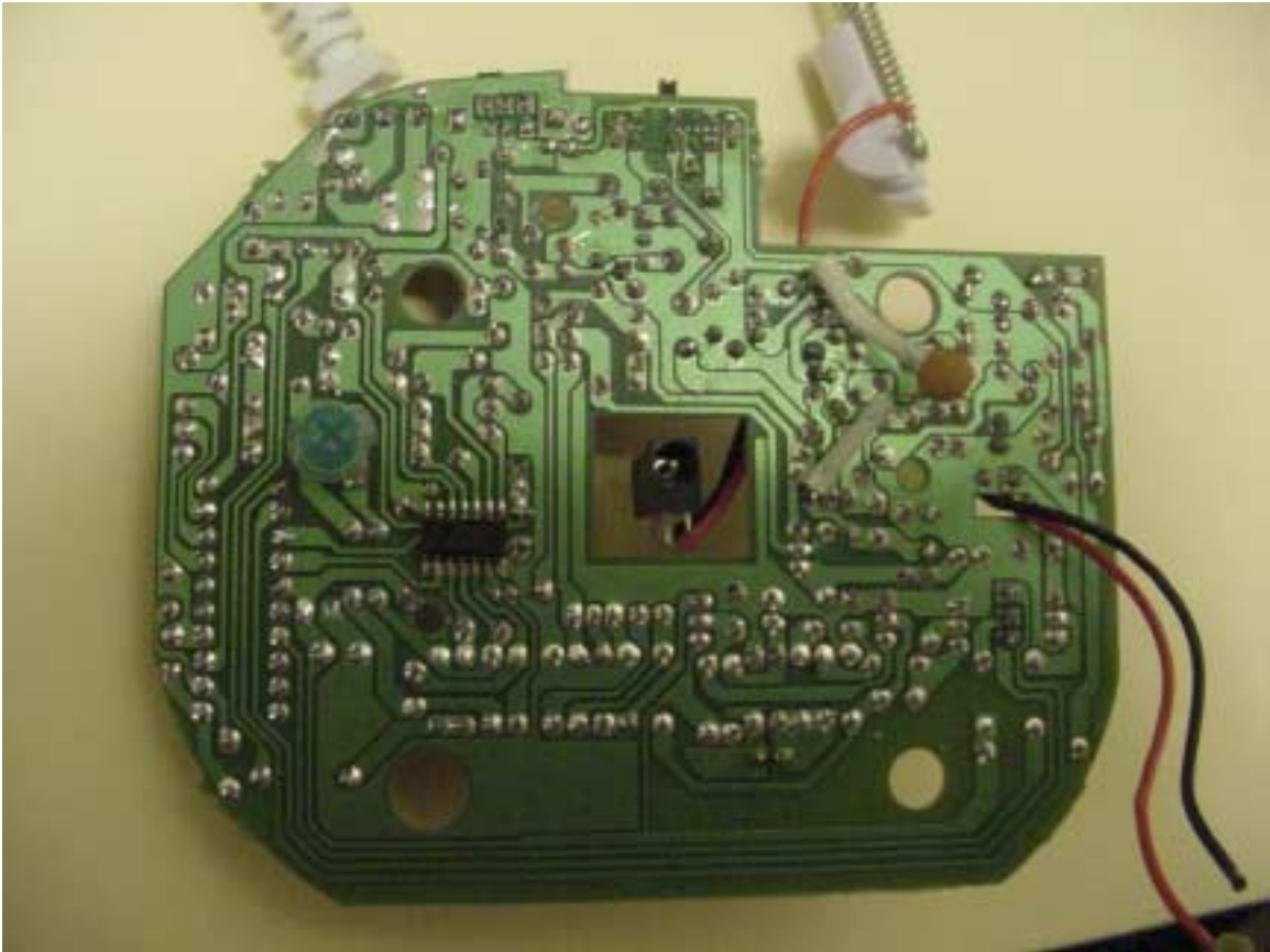
Solder Side of Motion Sensor/ RF board
