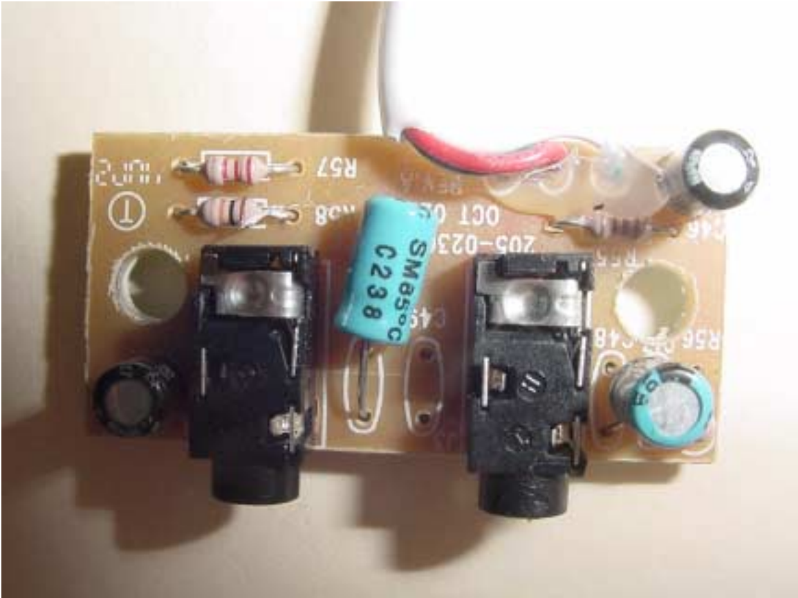
EUT Sensor Pad connector board Component Side
