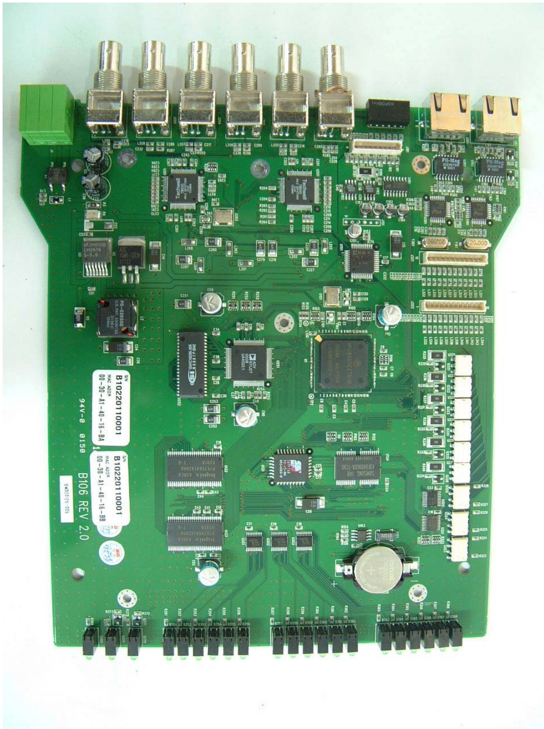
<FRONT VIEW OF MAIN BOARD>
