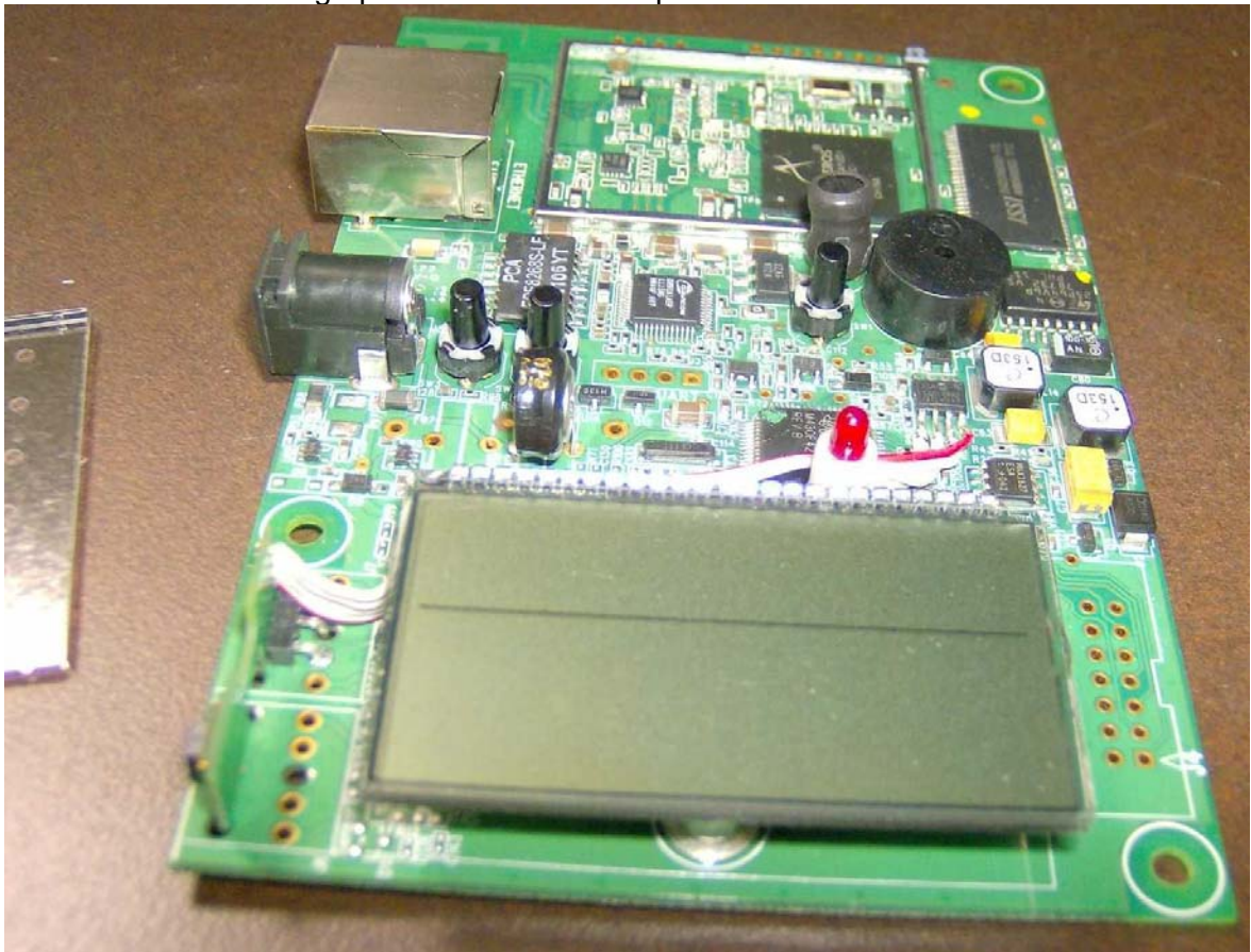
Photograph of PC Board: Component Side without shield
