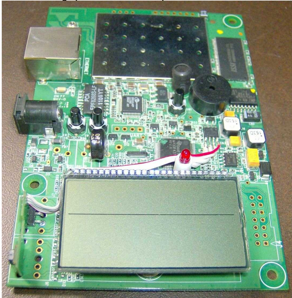
Photograph of PC Board: Component Side with shield
