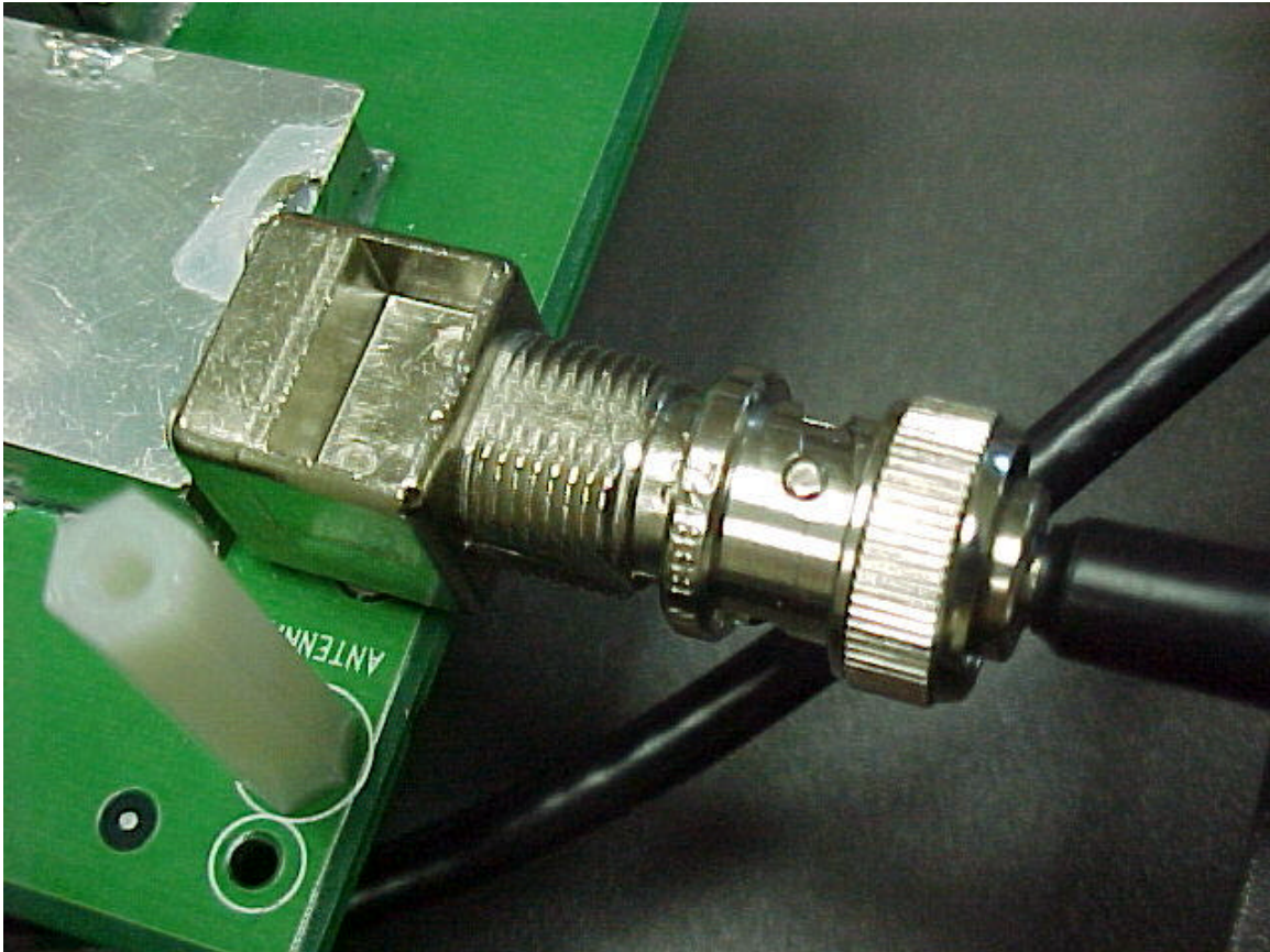
Photo Nine Single PCB showing Antenna Connection
