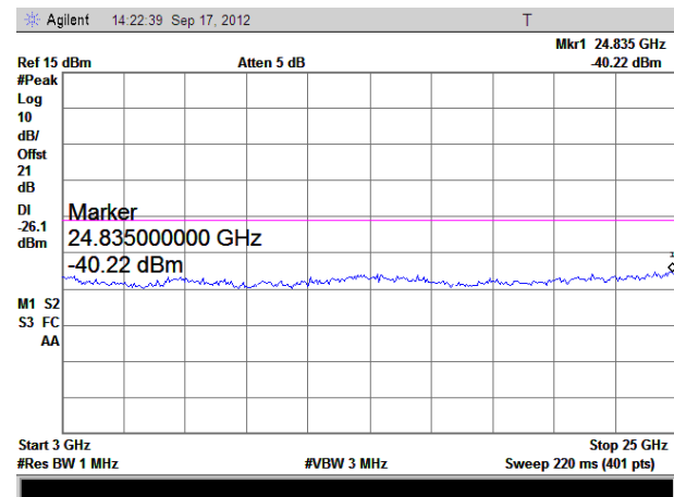
(Plot B.2: Channel = 19, 3GHz to 25GHz)
