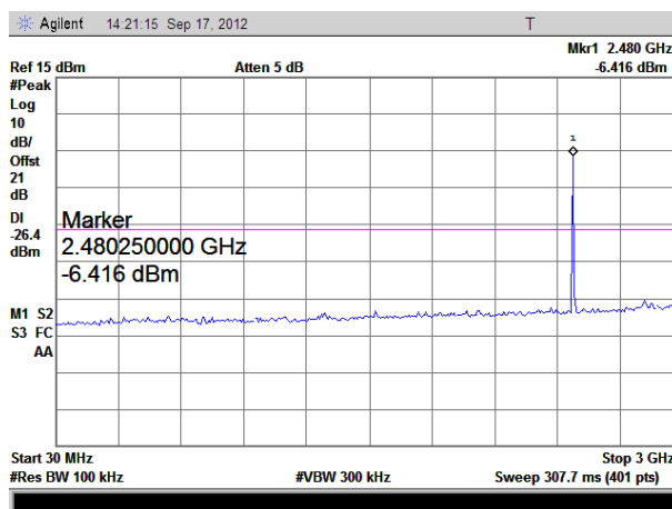
(Plot C.1: Channel = 39, 30MHz to 3GHz)
