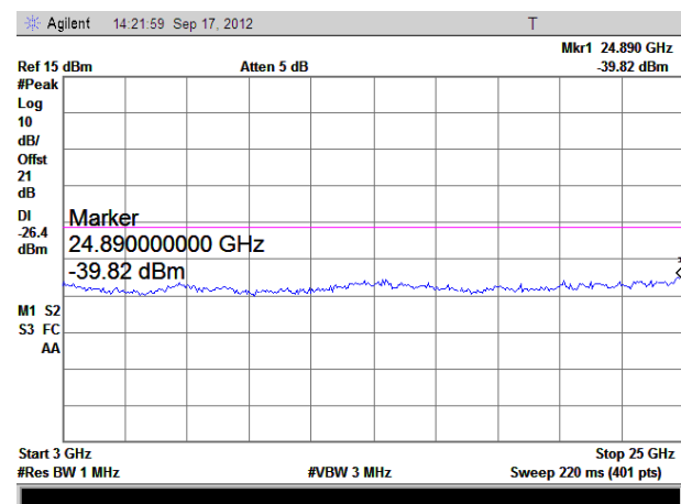
(Plot C.2: Channel = 39, 3GHz to 25GHz)
