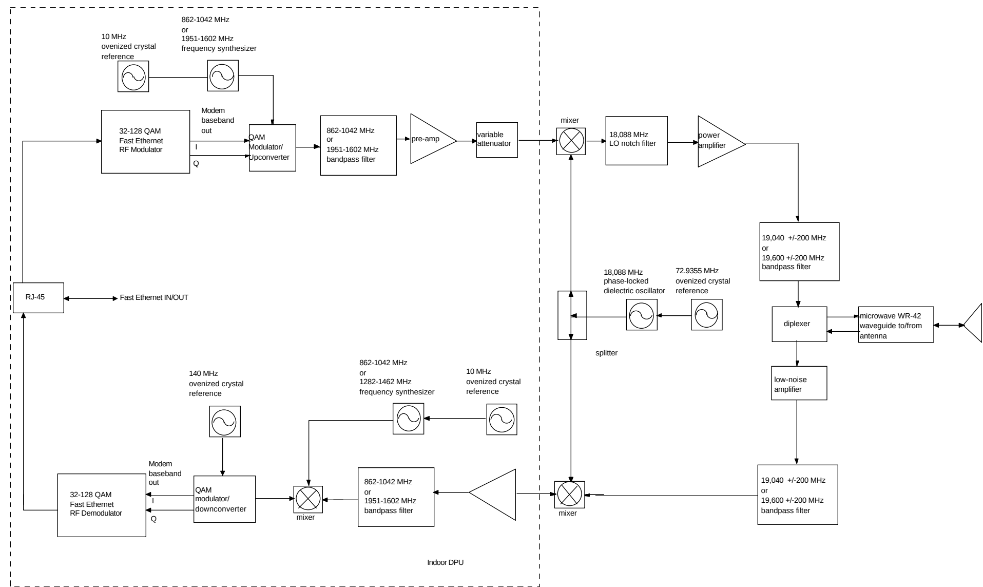
Block diagram of enet100 transciever
