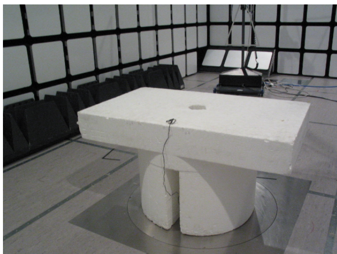
Picture 2 Radiated emission measurement Bluetooth TX
