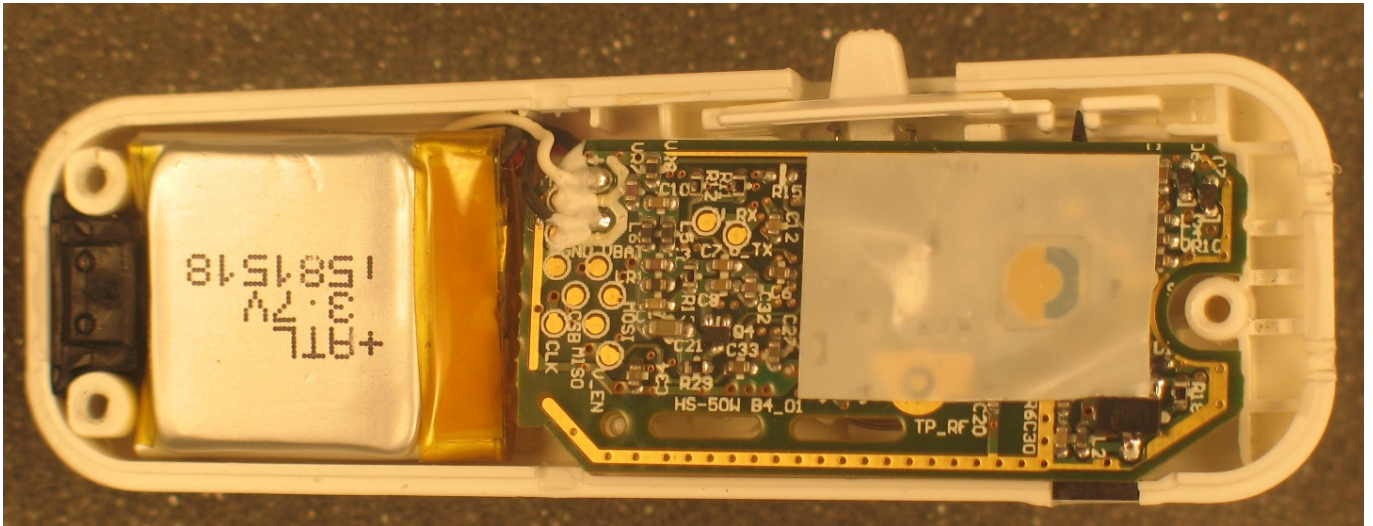
Picture 1. HS-51W internal picture.
