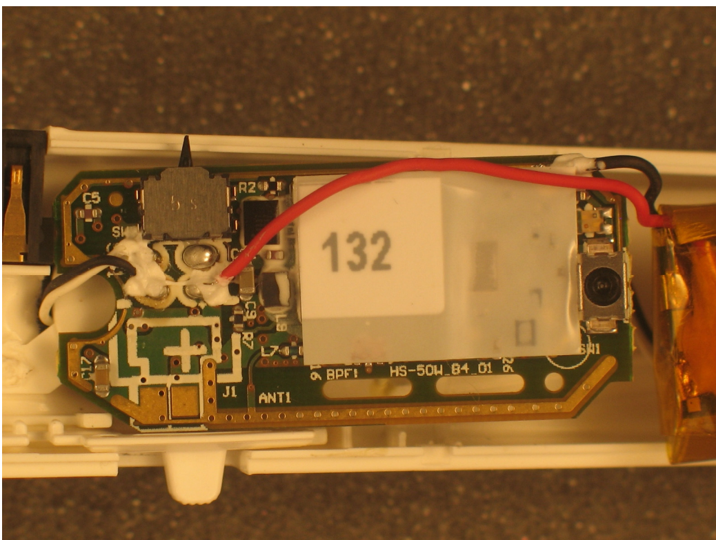
Picture 4. HS-51W PCB from back with PET-sheet.
