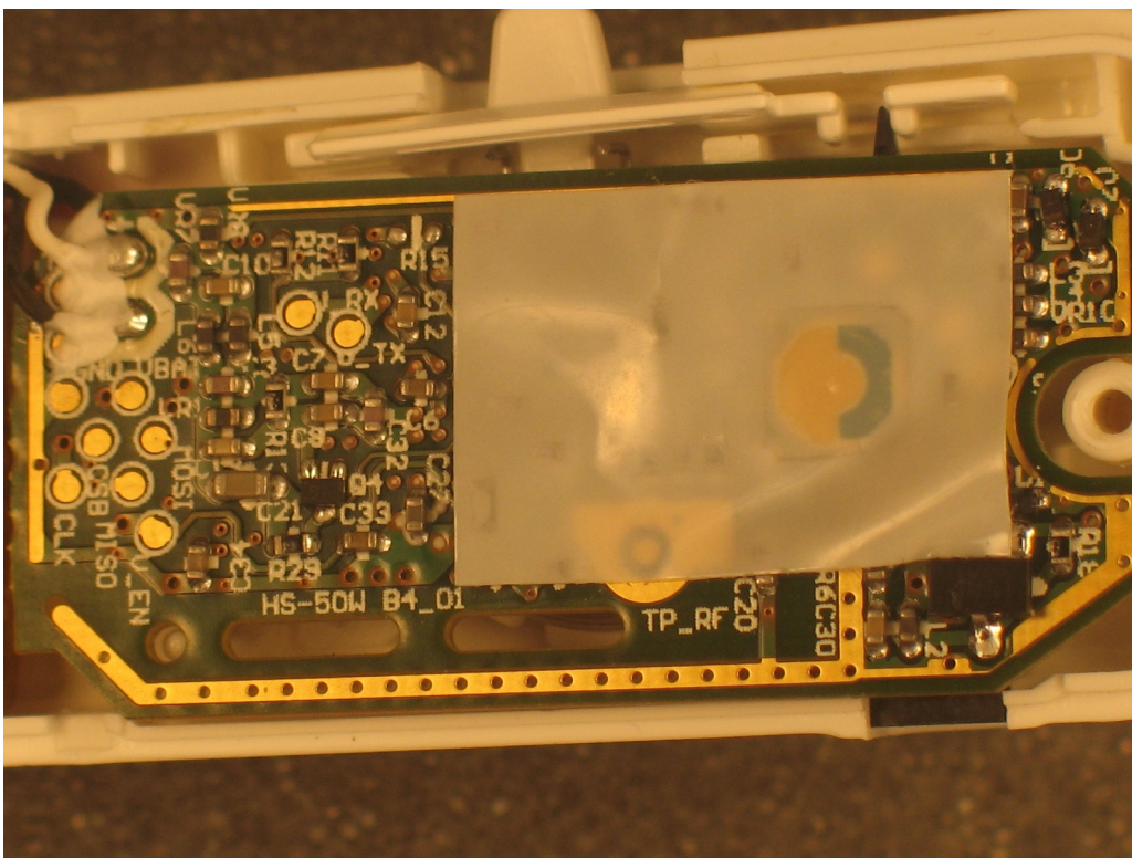
Picture 2. HS-51W PCB from front with PET-sheet.
