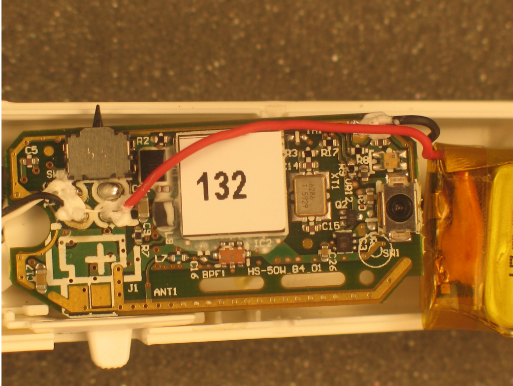
Picture 4. HS-51W PCB from back without PET-sheet.
