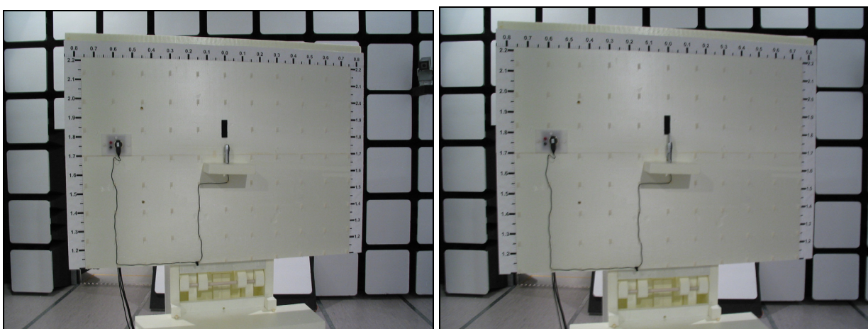
Picture 2 Spurious radiated emissions. Flap closed and open
