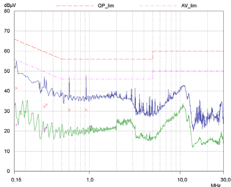
Picture 29: AC power line emissions, line N
