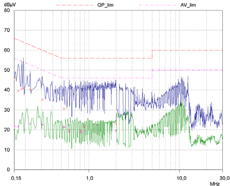
Picture 28: AC power line emissions, line L.
