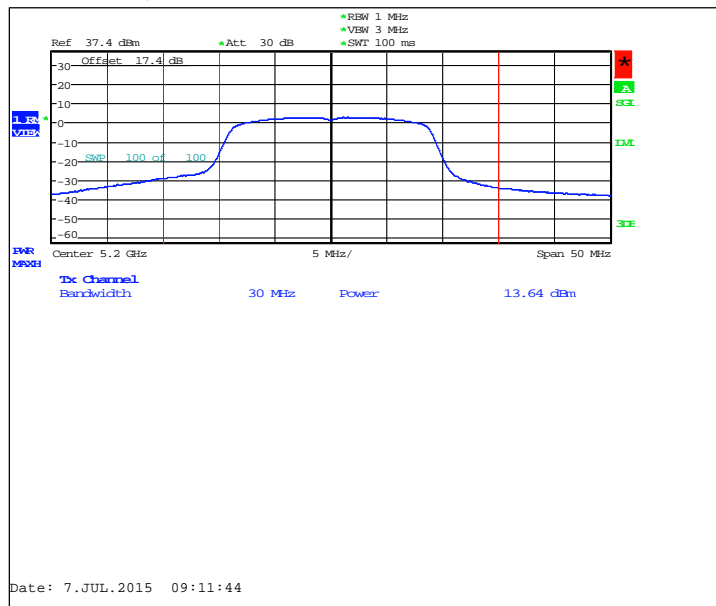
Channel 40 / 5200MHz
