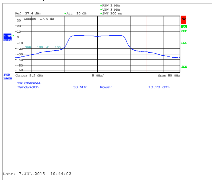
Channel 40 / 5200MHz
