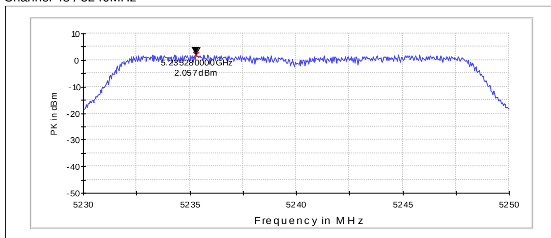
Channel 48 / 5240MHz
