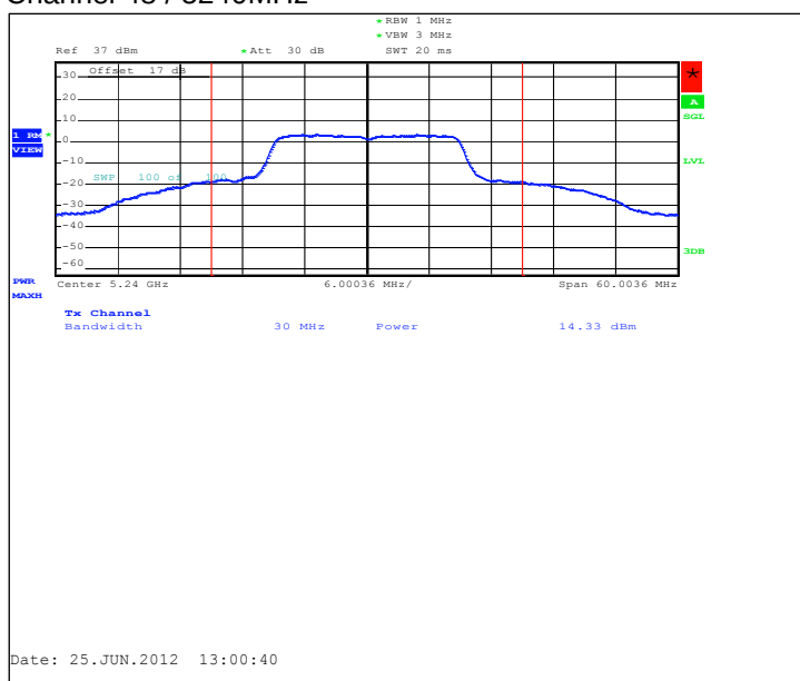
Channel 48 / 5240MHz
