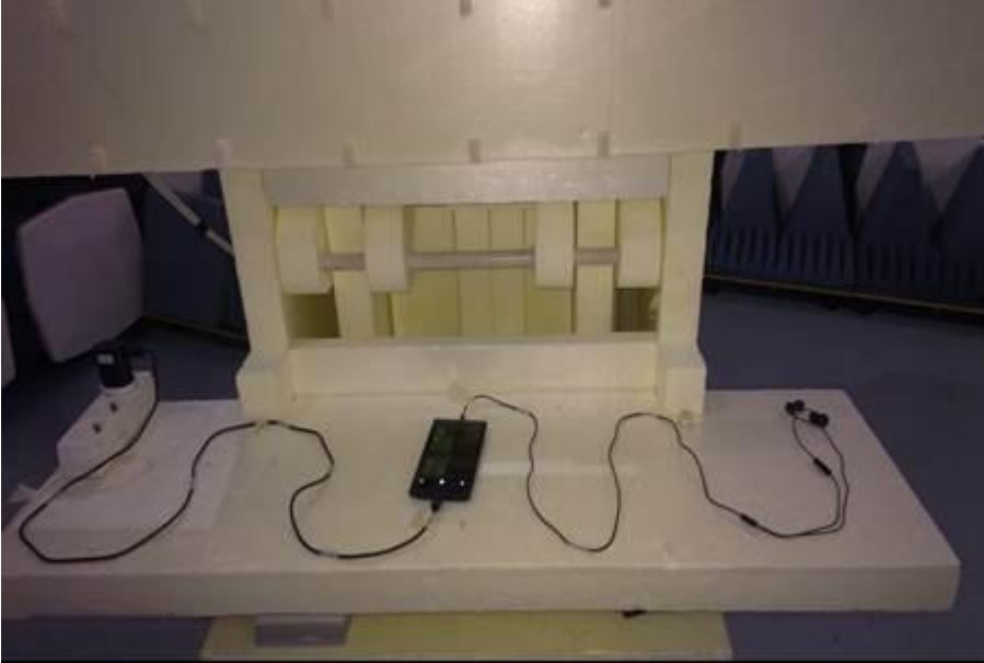
Picture 3. FCC Part 15B Radiated emissions
