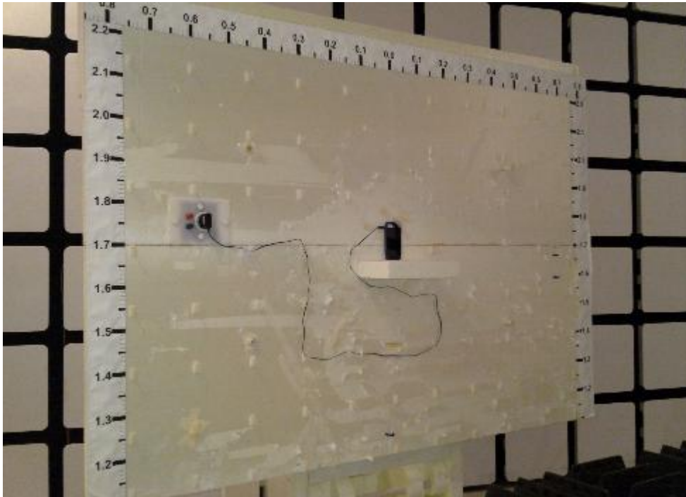
Picture 5. FCC Part 15C Radiated emissions FM TX
