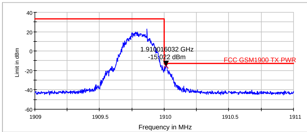
GSM, channel 810 / 1909.8 MHz (Peak detector, RBW: 3 kHz)
