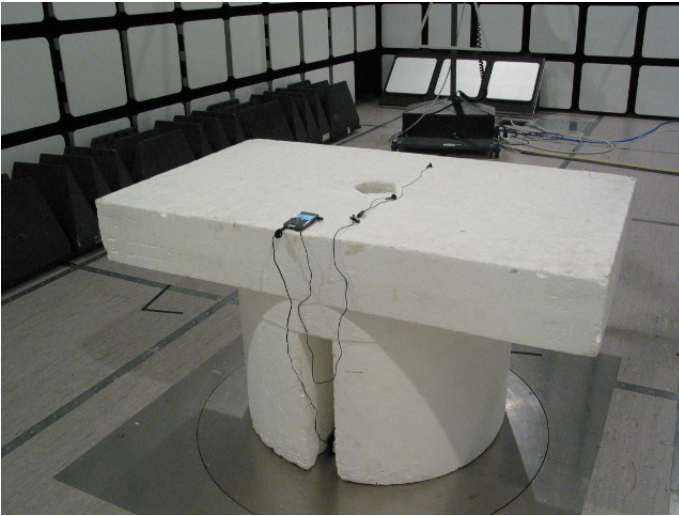
Picture 3 Radiated emission measurement GSM RX / FM radio on
