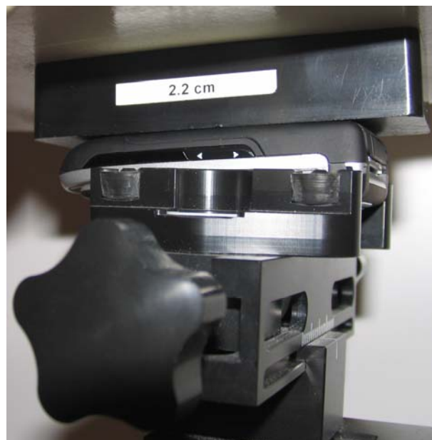
Photo of the device positioned for Body SAR measurement. The spacer was removed for the tests.
