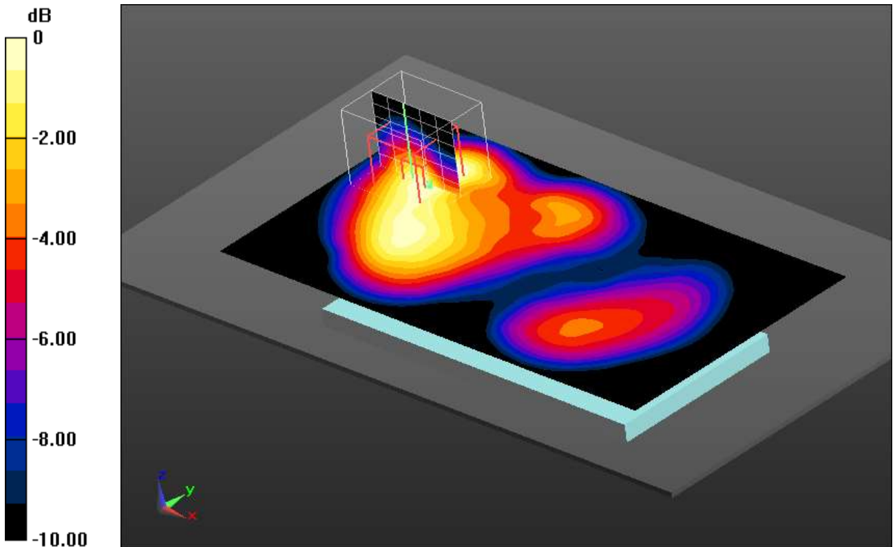
0 dB = 0.559 W/kg = -2.53 dBW/kg
