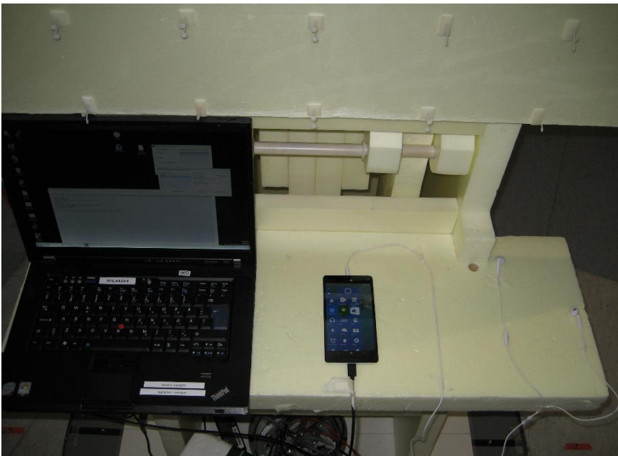
Picture 2. FCC Part 15B Radiated emissions
